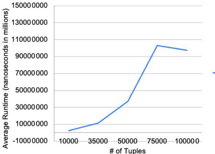
Join Case 1 - Natural Join (Average Runtime vs # of Tuples)
