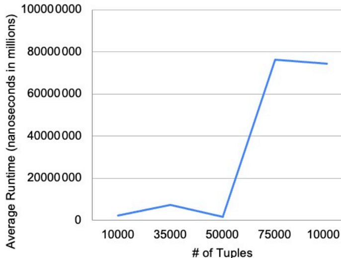
Join Case 2 - Equi-Join (Average Runtime vs # of Tuples)
