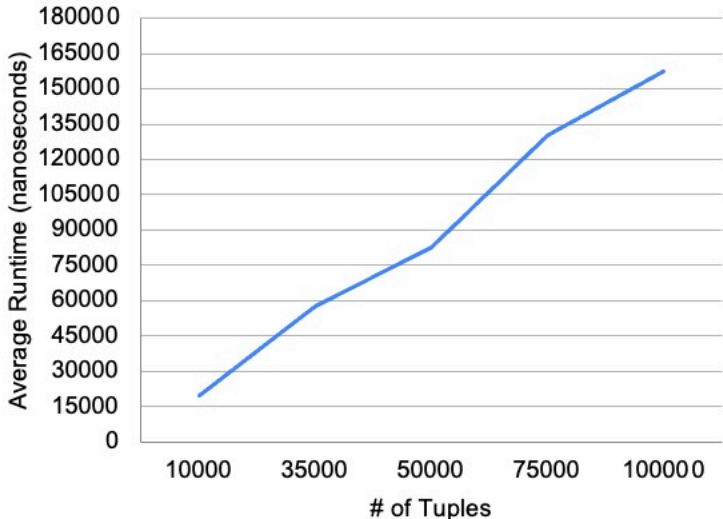
Select Case 1 - String (Average Runtime vs # of Tuples)
