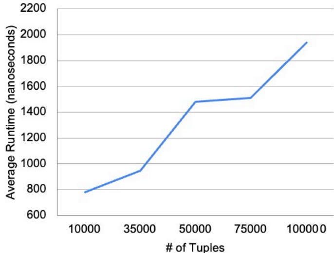
Select Case 2 - Predicate (Average Runtime vs # of Tuples)
